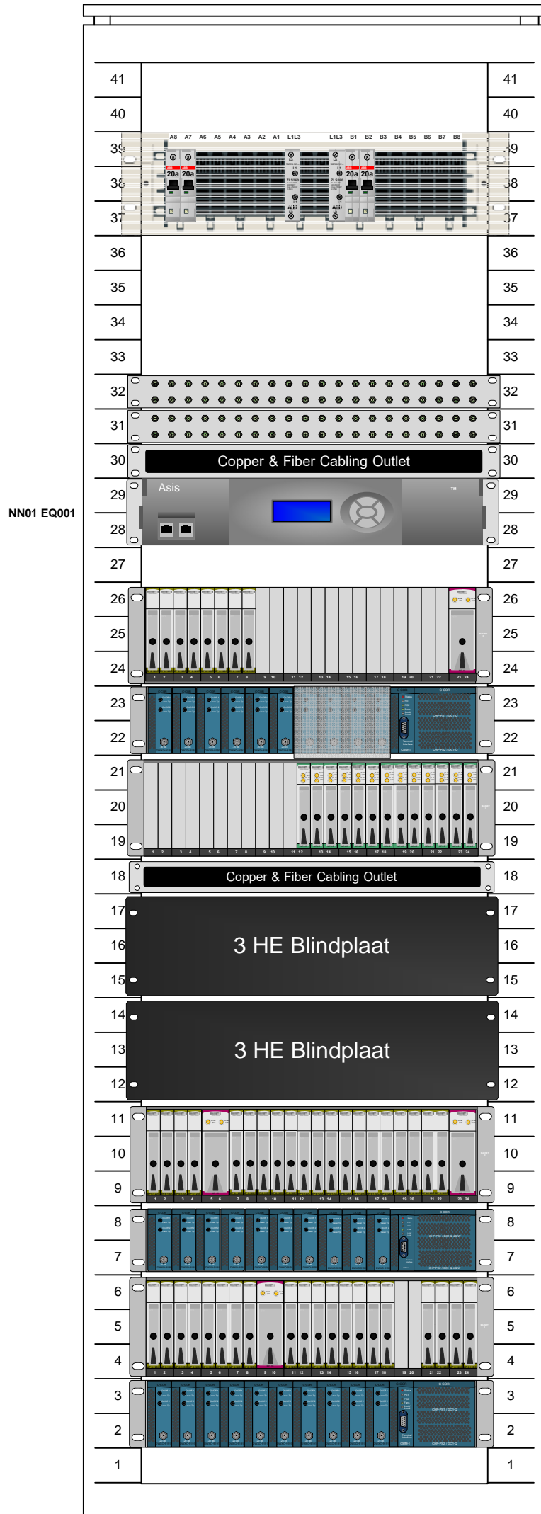
Front Elevation
