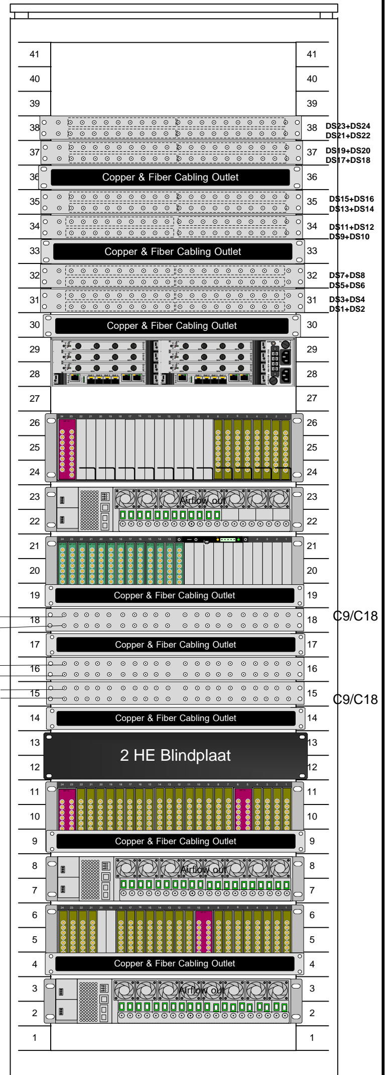
Rear Elevation
